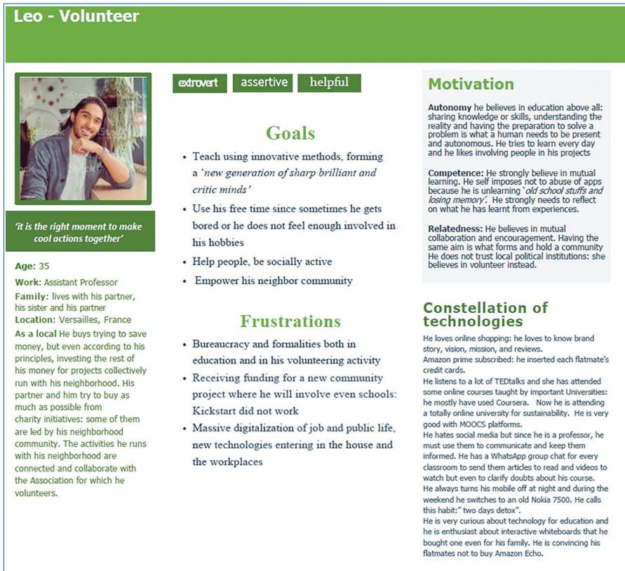
Figure 6.1. Persona volunteer.
