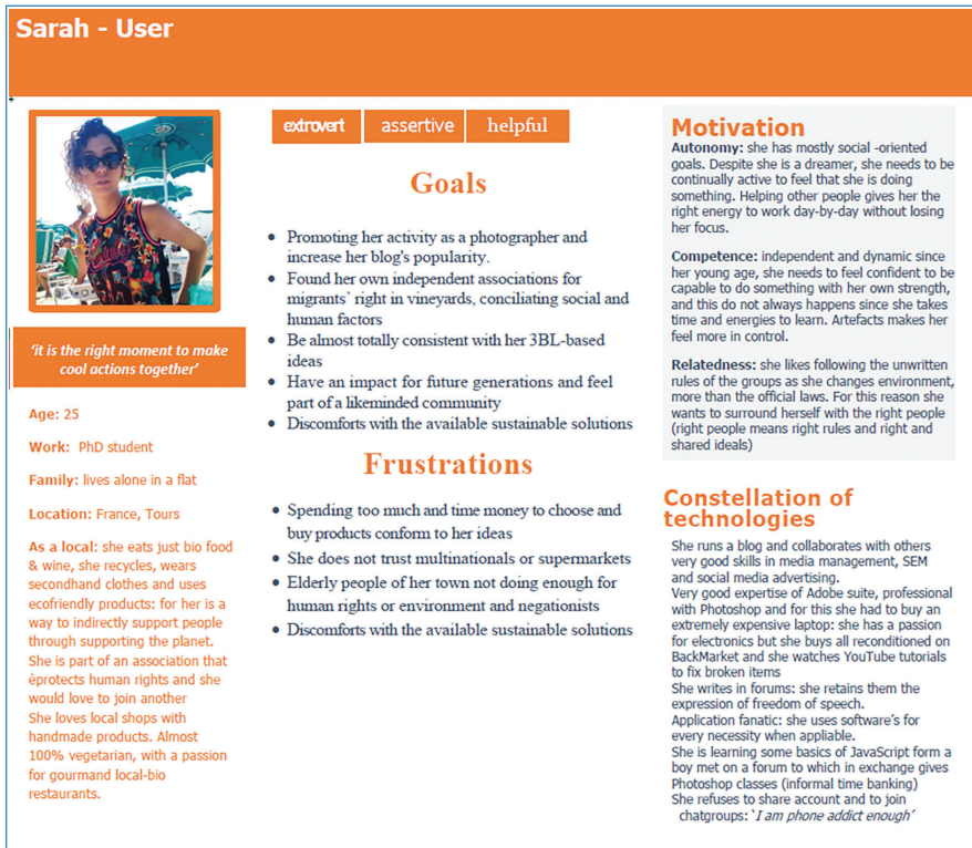
Figure 6.2. Persona user.
