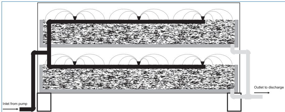
Figure 4.20. Biofiltro Wiggle Room treatment system, showing stacked containerised filters and separate control/pumping unit. Adapted from Biofiltro (2020b).
