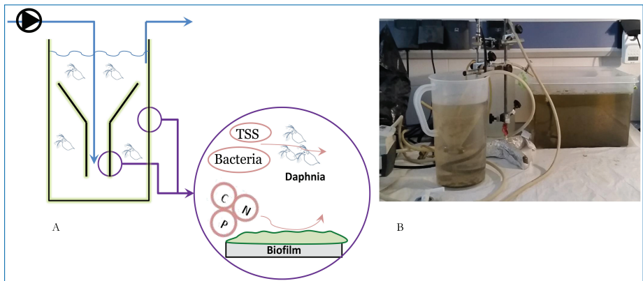
Figure 5.6. (a) Scheme of the Daphniafilter reactor used in the lab-scale experiments and (b) experimental set-up at lab scale. Adapted from Pous et al. (2020).
