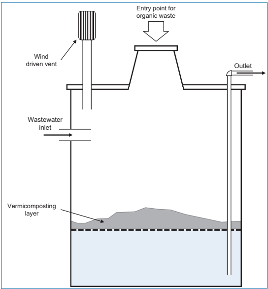
Figure 4.17. Worm Farm system, adapted from A&A Worm Farm Waste Systems (2020).
