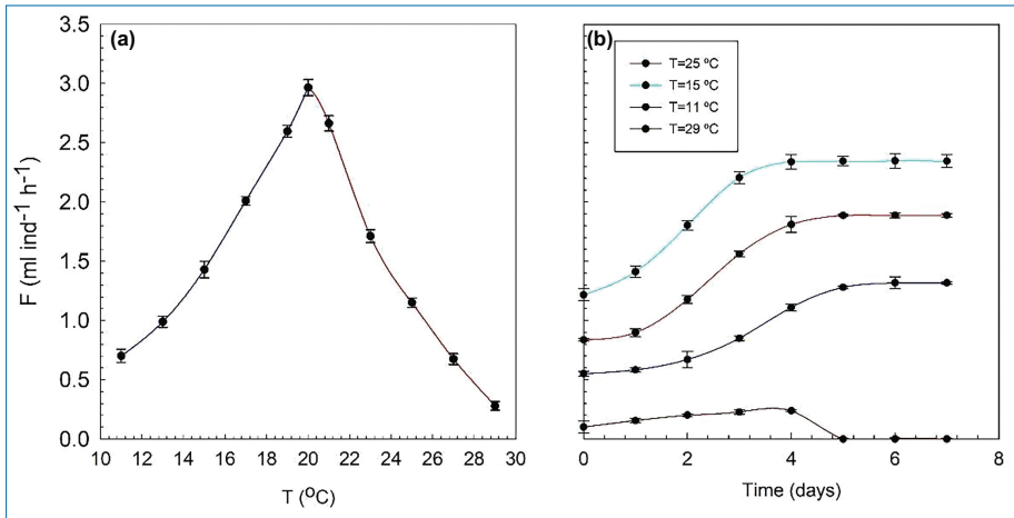
Figure 5.4. (a) D. magna filtration capacity, F (ml ind -1 h -1 ) versus water temperature and (b) D. magna filtration capacity F (ml ind -1 h -1 ) during acclimation versus the time (in days) exposed at each water temperature.
