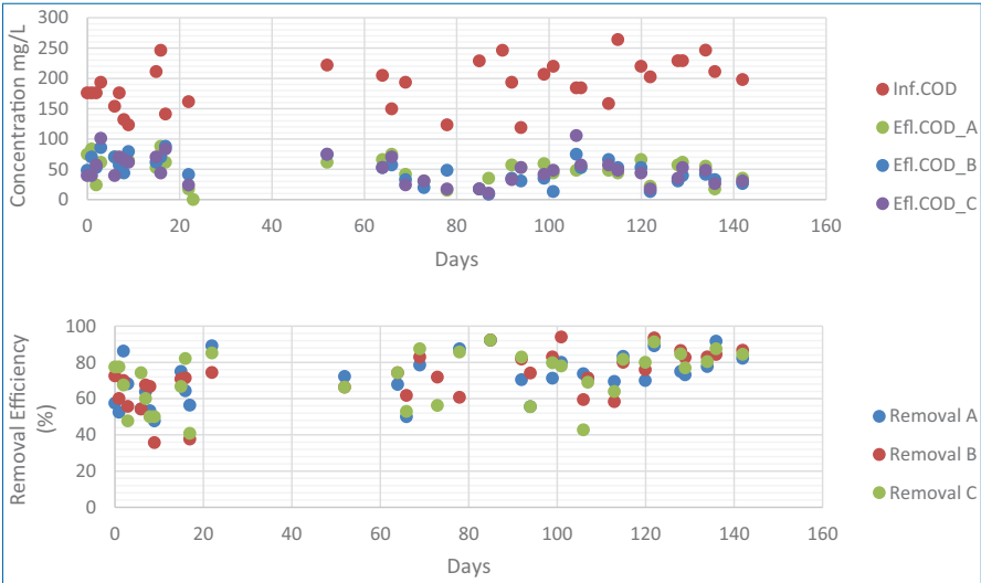
Figure 6.6. COD concentrations and removal performances for each of the tested platform designs. Note: A is the average data from the double cascade photobioreactors, B the thin layer cascade photobioreactors and C the single platform photobioreactors.
