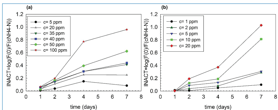
Figure 5.5. Inactivation factor (INACT) versus exposure time (in days) for the different chemical dosages c (in ppm = mg\ L^{-1} ) for (a) NH_4^+-N and (b) NO_2^--N .
