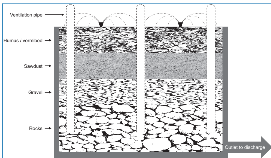
Figure 4.19. Sistema Toha®. Adapted from Sepúlveda (2004).
