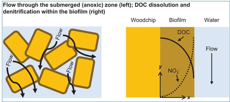
Figure 4.8. Principles of denitrification in a woodchip bioreactor. DOC = Dissolved Organic Carbon. Adapted from Lopez-Ponnada et al. (2017).
