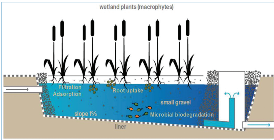
Figure 3.4. General mechanisms for the removal of pollutants in CWs, adapted from Gorito et al. (2017); Tilley et al. (2008).
