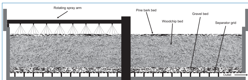
Figure 4.21. Cross-sectional representation of the vermifilter at Combaillaux, adapted from Naigeon (2005).
