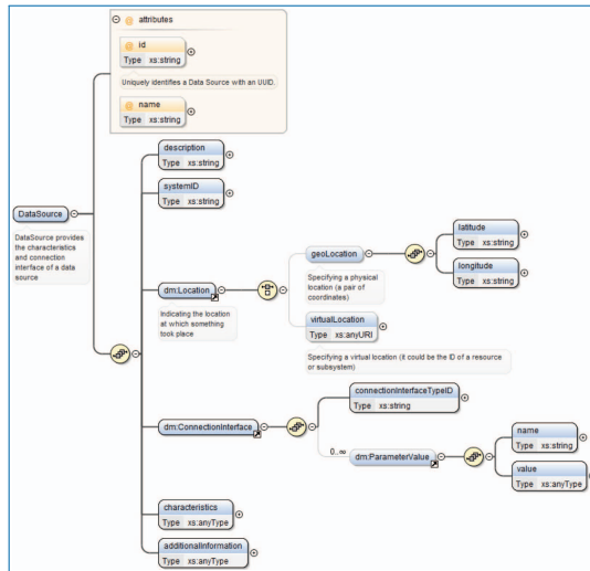
Figure 2.4. Data source entity modelling.
