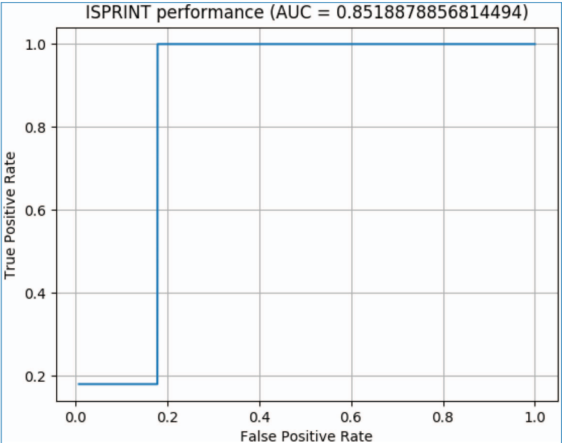
Figure 3.8. ROC curve of the CloudCare2U classifier.
