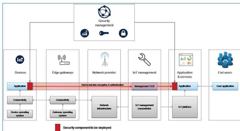
Figure 12.8. Security components.
