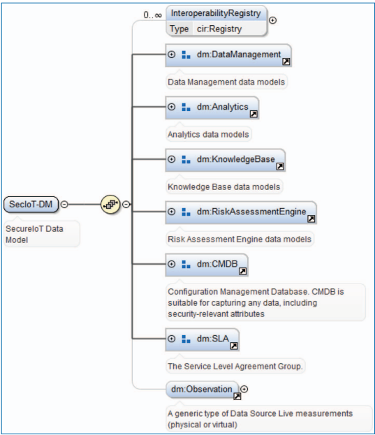
Figure 2.2. Logical groups of the SecureIoT data models.
