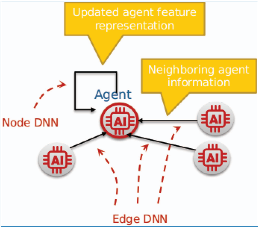
Figure 5.2. The procedure for updating the feature representations of the edges and nodes visible by each agent. The edge Deep Neural Network (DNN) takes as input the previous edge feature values and the adjacent agent features, and updates the feature representation of each edge. The node DNN aggregates the information from the updated edge feature values, and updates the feature representation of the specific node.
