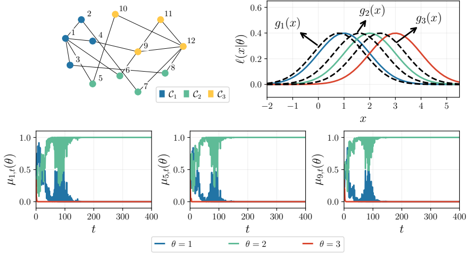
Figure 5.1: (Top left) Network topology showing the different clusters \mathcal{C}_c corresponding to Example 5.3. The graph is undirected and there are no self-loops. (Top right) Likelihood models \ell(x|\theta) (solid line) and true models g_c(x) (dashed line). (Bottom) Belief evolution over 400 iterations for agents 1, 5, and 9. We see that, as t grows, the agents place their full belief mass on the unique minimizer \vartheta^* = 2 .
