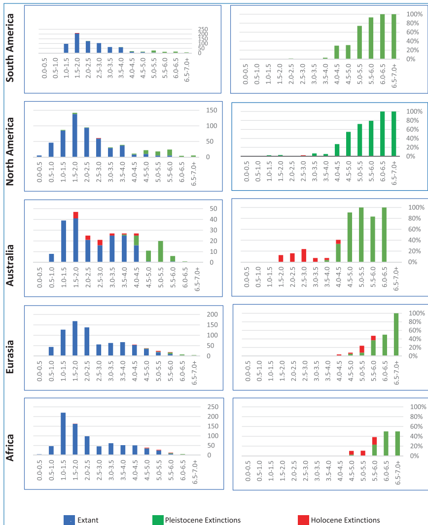
Figure 4.4. Mammal species extinctions per body weight and per continent in absolute numbers (left) and in relative numbers (right). Body weights (horizontal axis) are in 10\log , e.g., the category 1.0-1.5 includes mammals with body weights from 10 to 32 grams. The data are from Table S6 in [527] and updated Figure 1 in [306]. Some of the extinctions in red (Holocene) may have occurred after (partially) transitioning from hunting and gathering to agriculture.
