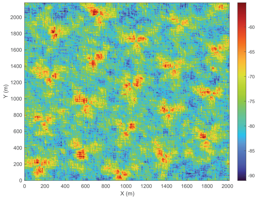
Figure 6.17. Radio environment map showing the path loss with a resolution of 5 m \times 5 m.
