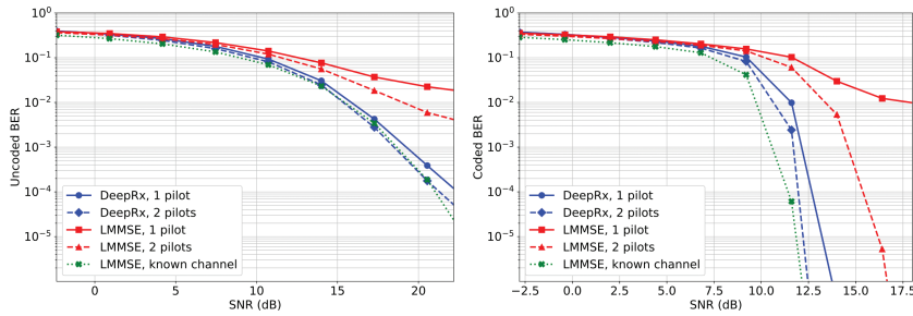
Figure 5.25. DeepRx MIMO can surpass the LMMSE receiver in TDL-E channels and reach near LMMSE with known channel performance.
