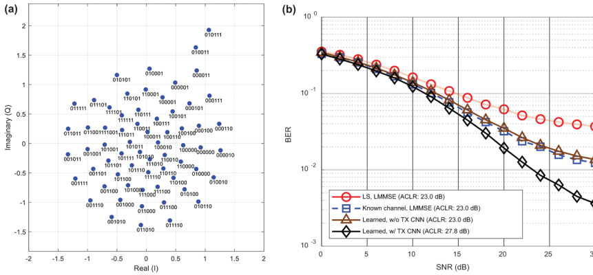
Figure 5.27. (a) An example of a learned constellation shape, and (b) the corresponding BER under a nonlinear PA.
