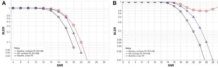
Figure 5.20. Performance of the AI-empowered receiver.
