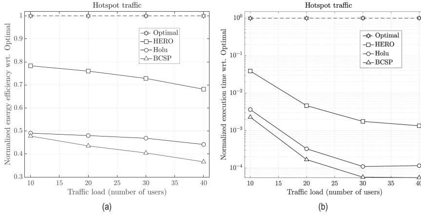
Figure 6.10. Normalized energy efficiency (bits/joule, linear scale) and execution time (s, logarithmic scale) of all studied algorithms with reference to the optimal solution for different traffic load conditions [40].
