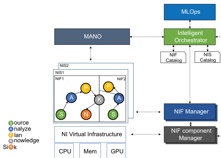
Figure 5.7. The NI orchestration framework.
