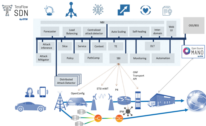
Figure 5.12. Enabling NI in the cloud-native SDN controller.
