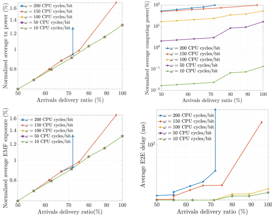
Figure 6.12. Trade-off involving communication, computation power, EMF exposure, data delivery ratio, and E2E delay.
