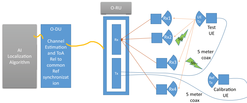
Figure 4.3. Setup for ultra-accurate UE distance measurement.
