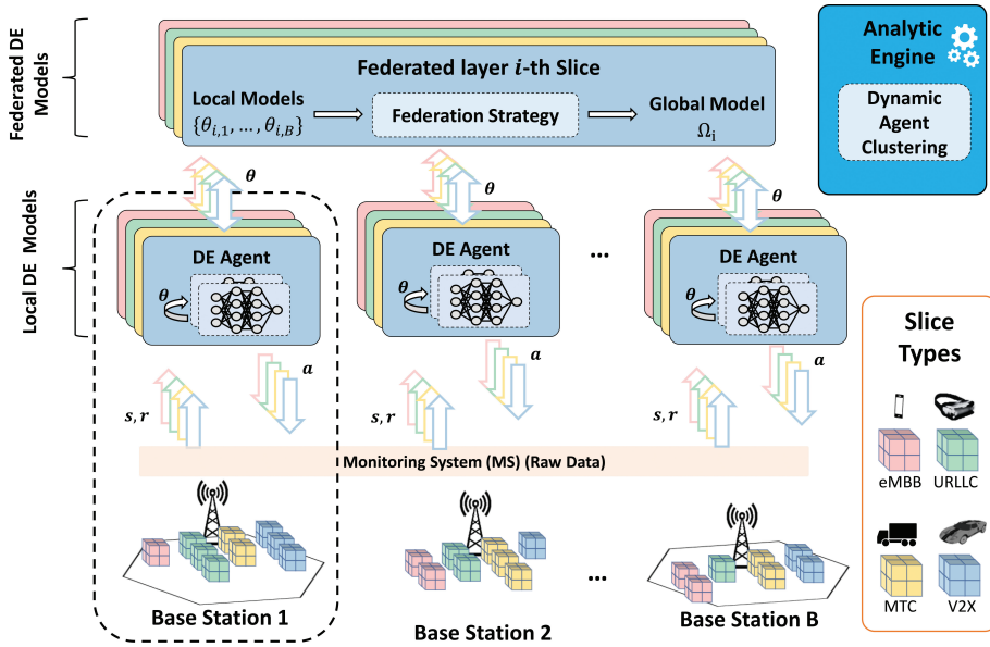
Figure 5.38. Generic federated DRL architecture for RAN slicing [49].
