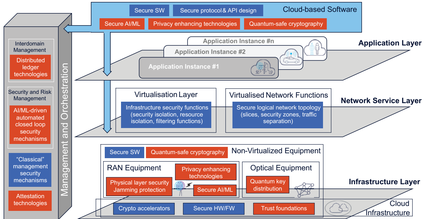
Figure 2.6 Overview of the essential 6G security architectural components [33]. The new 6G security technology enablers highlighted in red, and the more traditional building blocks are in blue.
