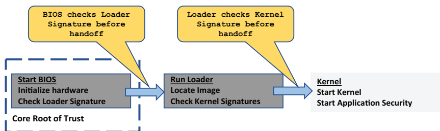
Figure 8.5. Secure boot execution flow.
