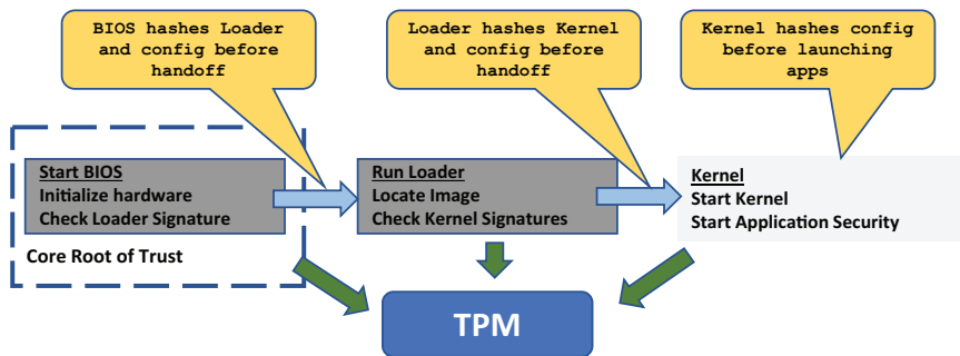
Figure 8.6. Measured boot execution flow.
