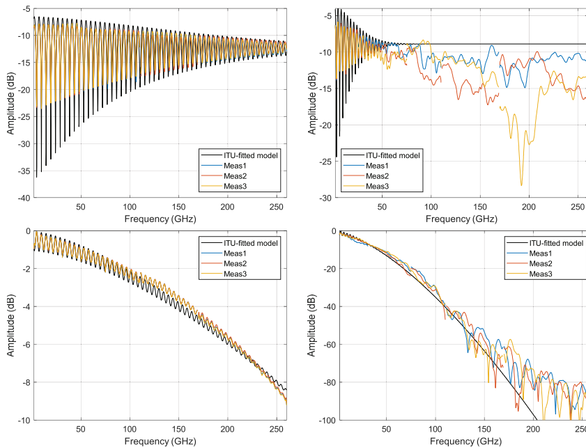
Figure 3.46. Material reflection (line a) and transmission gain (line b) compared with the ITU-fitted model fitted by measurement. The measurement is performed at three different points separated by 10 cm on the slab.
