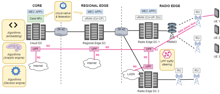
Figure 6.1. Overview of the sustainable virtual elastic edge computing architecture [17].
