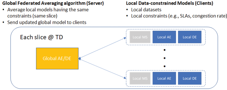
Figure 5.37. FL-based decentralized AEs for slice n .
