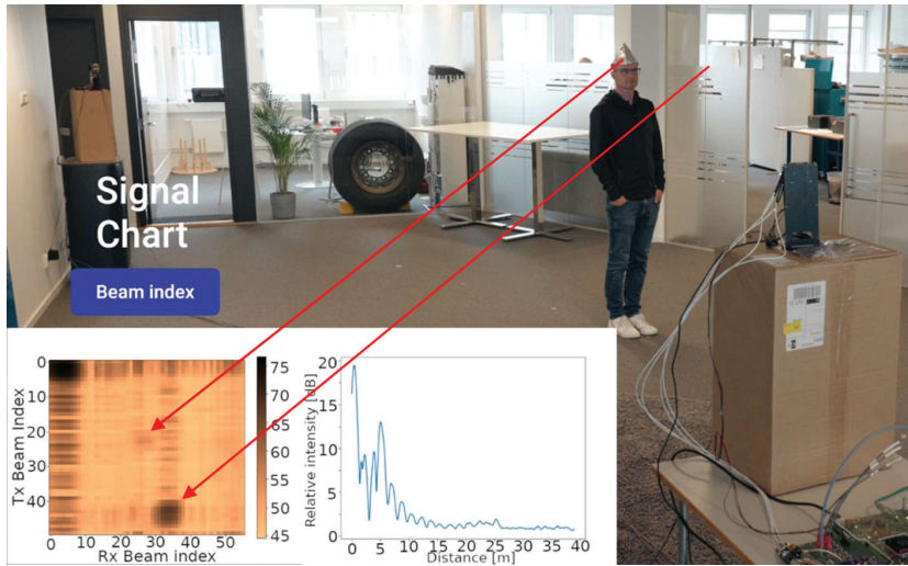
Figure 4.28. Initial demonstrations of JCAS using a bistatic setup at 69 GHz.
