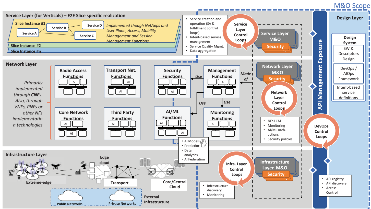
Figure 2.7 Proposed 6G management & orchestration system – structural view [34].
