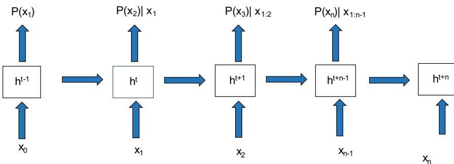
Figure 5.41. Probabilistic classifier for predicting anomalous sequences.
