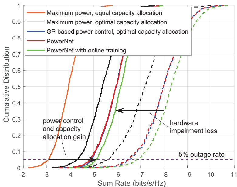
Figure 5.34. Sum rate performance comparison between proposed method (PowerNet) and baseline (optimization-based) with and without hardware impairments in the transceivers. Dashed lines: Ideal transmitters and receivers without hardware impairments. Solid lines: With hardware impairments in the transmitters and receivers.
