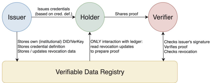
Figure 8.3. Roles that interact in a verifiable credential ecosystem.
