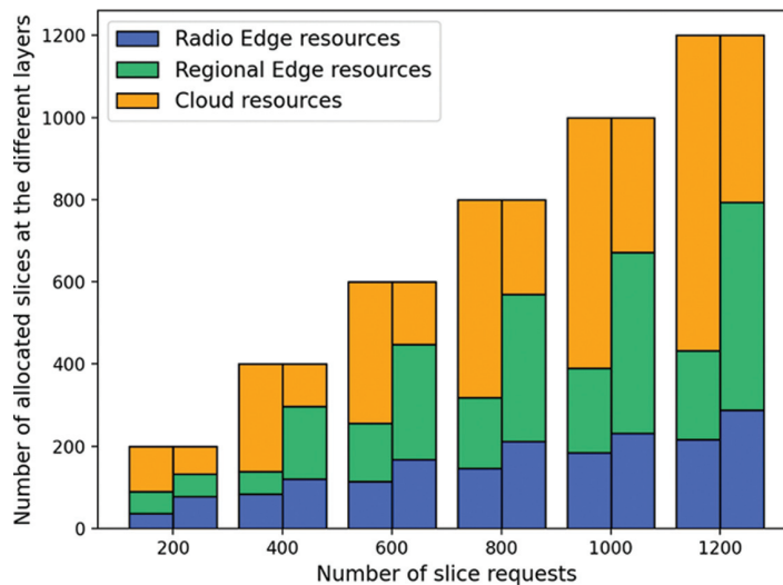
Figure 6.6. Number of allocated slices at the different computing layers for the proposed methodology when the objective is the minimization of the cost (left bar) and the minimization of the average latency per slice (right bar) for various number of slice requests.
