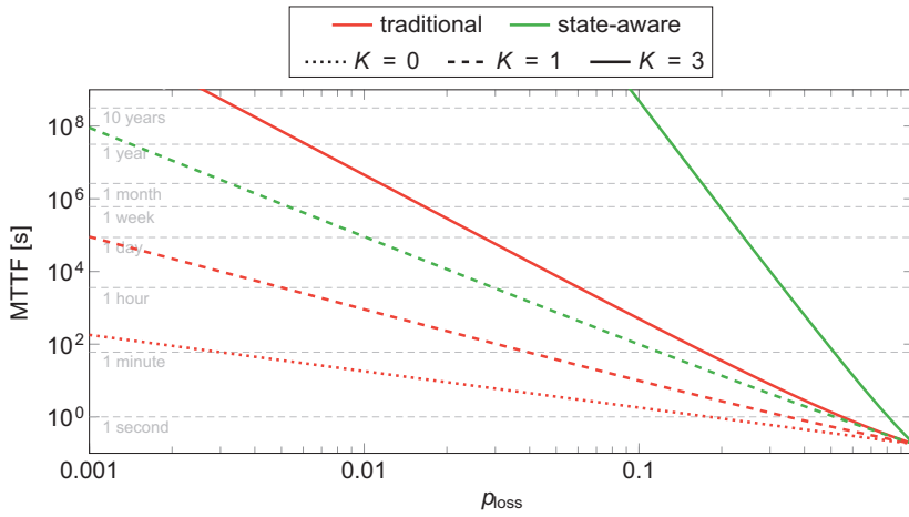
Figure 6.16. State-aware resource allocation allows increasing the mean time to failure by orders of magnitude while preserving low resource and energy consumption.
