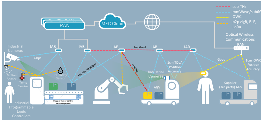
Figure 4.1. Expected sensing use cases in an Industry 4.0.
