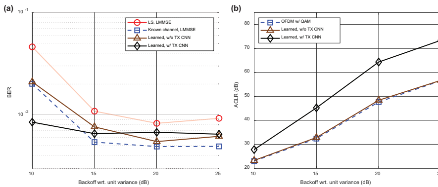
Figure 5.28. (a) BER of the different schemes with respect to the PA input backoff when the SNR is fixed at 24 dB, and (b) ACLR of the different schemes with respect to the PA input backoff. Note that here the PA backoff is defined with respect to unit variance, i.e., it represents the power of the PA input signal (not to be confused with PA backoff with respect to 1 dB compression point).
