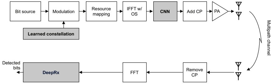
Figure 5.26. E2E learning for constellation shaping and out-of-band emission reduction.
