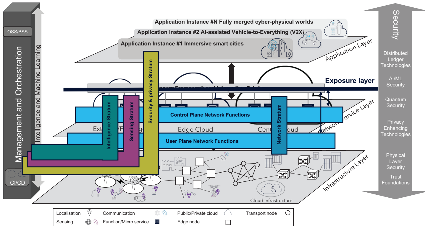
Figure 2.5 Functional view of the proposed 6G reference architecture with the focus on the stratus.
