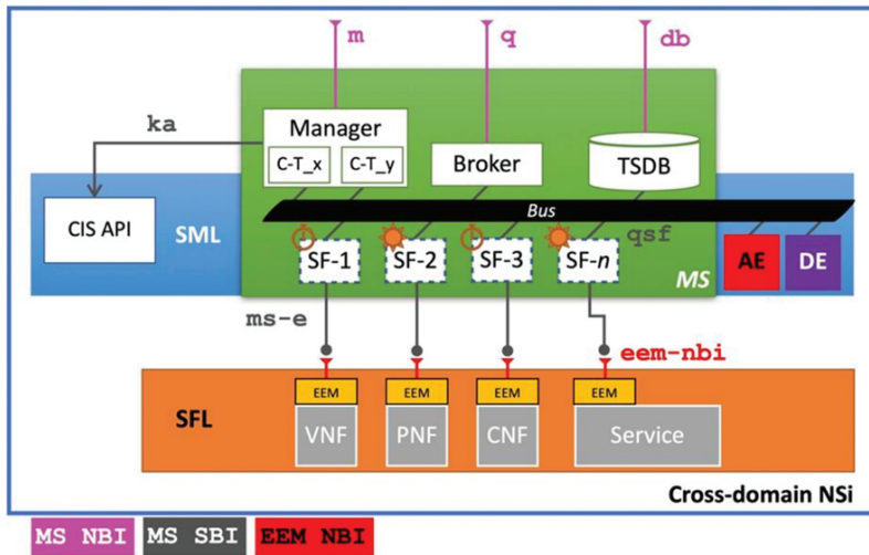
Figure 5.10. MANO-MS: Monitoring system of the proposed distributed and scalable MANO framework.
