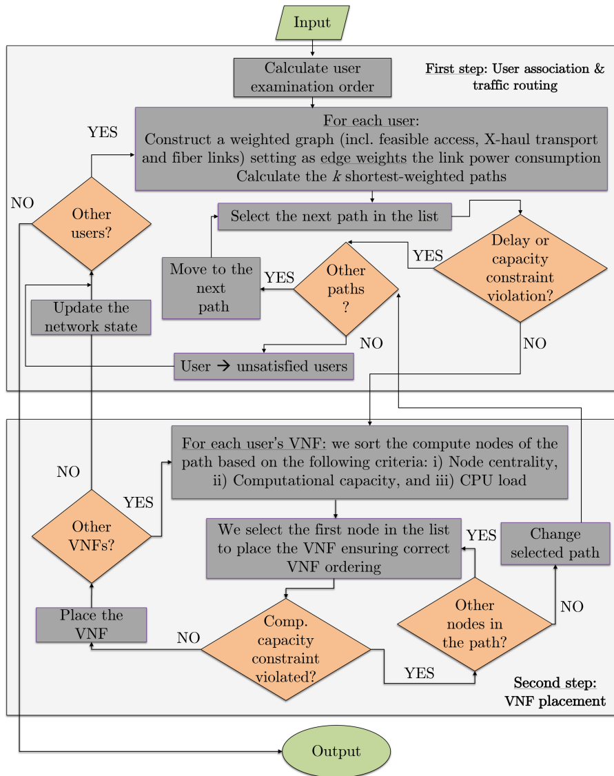
Figure 6.9. Flowchart of the proposed energy-efficient VNF placement, traffic routing, and user association algorithm (HERO) [40].
