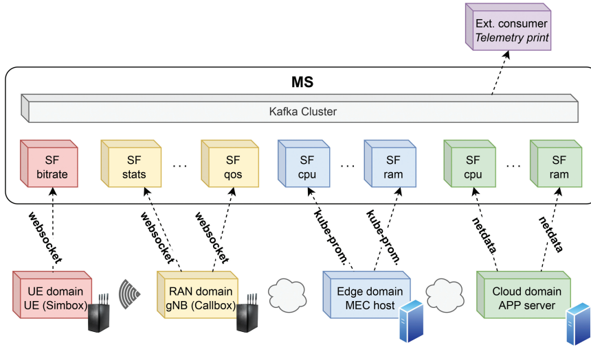
Figure 5.11. Multi-domain slice for 5G end-to-end monitoring.
