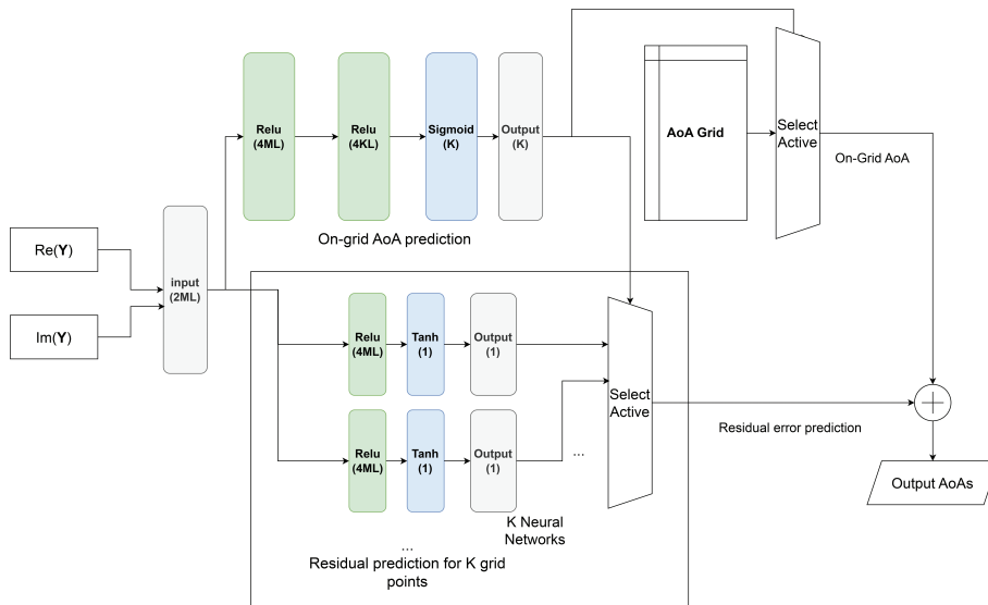
Figure 5.32. NN architecture for AoA prediction.
