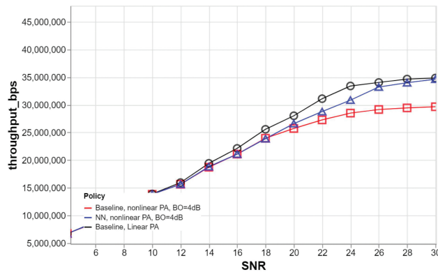
Figure 5.21. Achievable throughput with adaptive modulation and coding for AI-empowered receiver.
