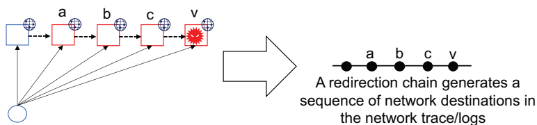
Figure 8.1. Example of redirection chain in malware distribution.
