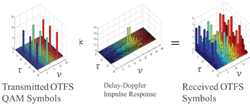
Figure 4.10. Transmitted OTFS QAM symbols and corresponding received symbols via delay Doppler channel.
