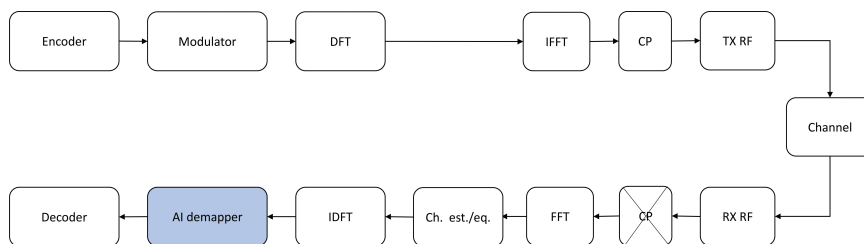
Figure 5.19. The radio transceiver architecture with AI-empowered receiver.
