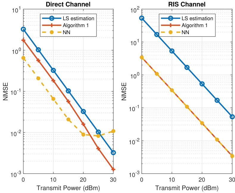
Figure 5.33. Comparison of performance of proposed methods with LS estimation for both direct and reflected channels, in the off-grid case.
