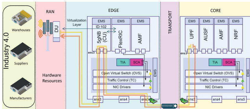
Figure 7.8. E2E programmable data path and data path network slicing.
