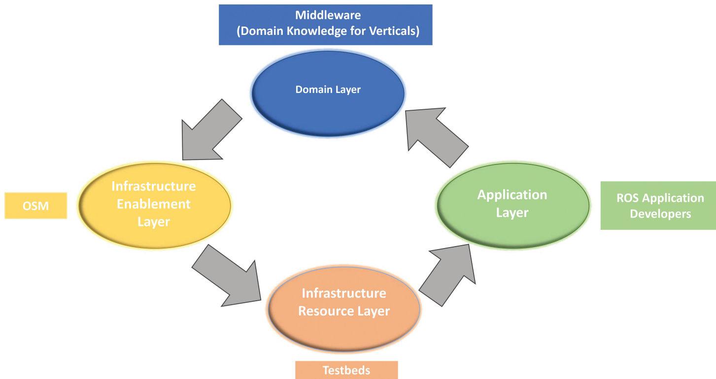
Figure 7.20 Interconnected layers.
