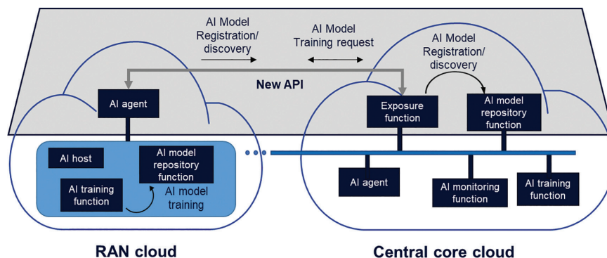
Figure 5.2. Architecture enablers for supporting AlaaS.
