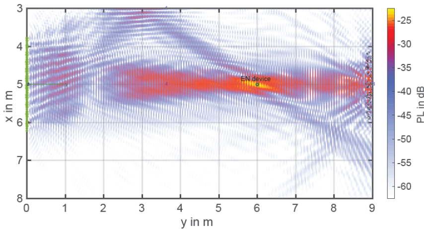
Figure 6.3. Illustration of the spot focusing of distributed beamforming towards the energy-neutral device.
