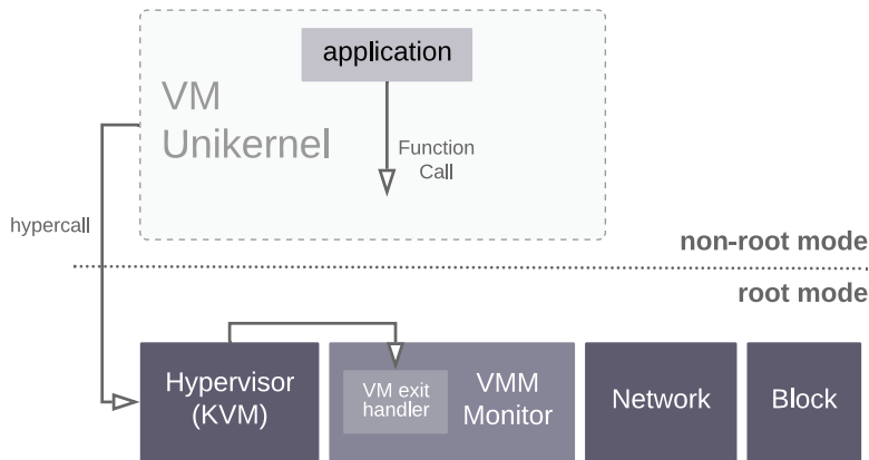
Figure 8.4. A unikernel running as a VM on HEDGE.
