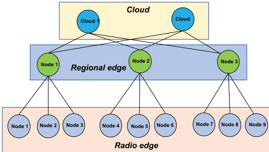
Figure 6.5. The multi-layered computing infrastructure under study.
