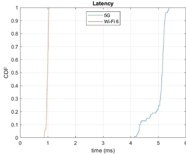
Figure 3.29. Latency of 5G and Wi-Fi 6 in the proposed testbed [81].
