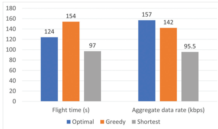
Figure 6.18. Flight time and aggregate data rate for the optimal, greedy, and shortest UAV trajectory.
