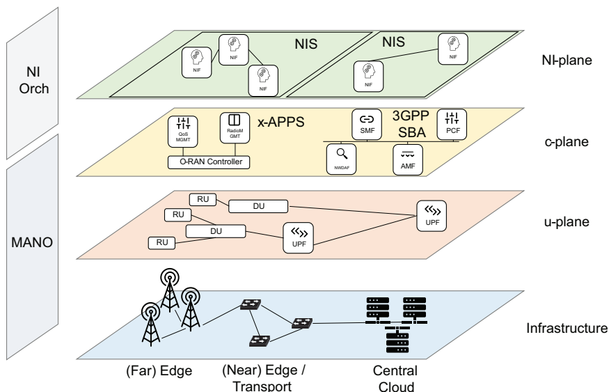
Figure 5.4. The framework for the NI integration in the overall architecture.
