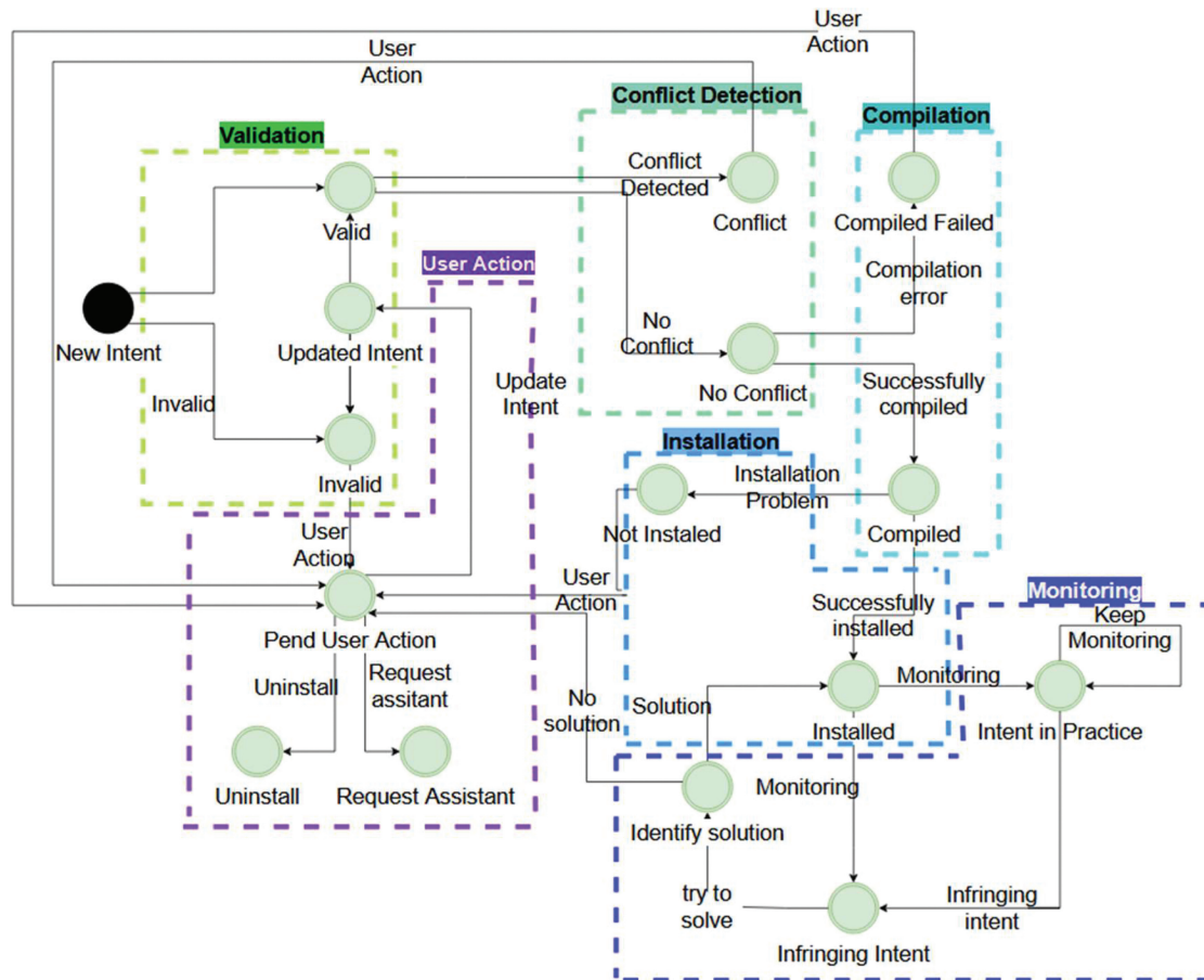
Figure 7.19 State machine for enabling IBN.
