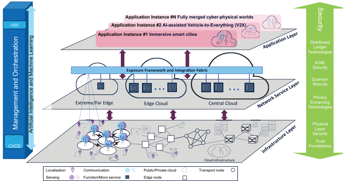
Figure 2.4 End-to-end system view of the 6G architecture [23].
