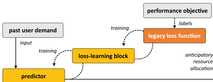
Figure 5.15. Loss meta-learning for NI.
