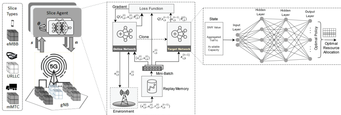
Figure 5.39 An illustration of local DDQN workflow.
