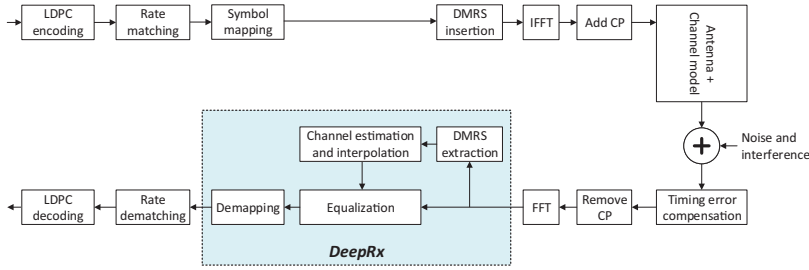
Figure 5.22. DeepRx replaces most of the processing blocks in the frequency domain receiver processing in the physical layer. The blocks inside the DeepRx box describe the traditional receiver processing blocks that DeepRx replaces with a trained neural network.
