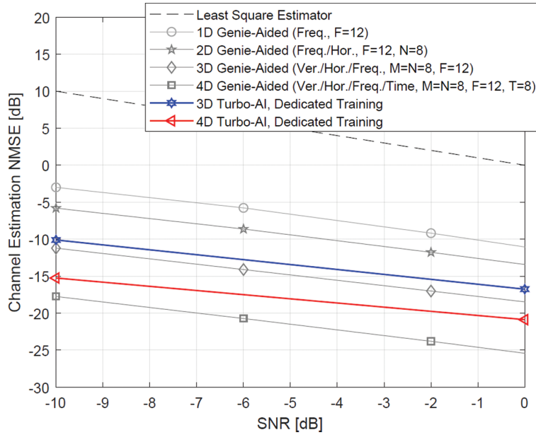
Figure 5.31. Comparison of the proposed ChE schemes, turbo-AI, with the statistically optimal solution MMSE-based estimator. The MMSE estimator for the above results included a 6144 \times 6144 matrix inversion operation.
