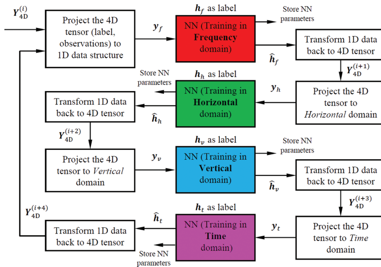
Figure 5.30. The neural network architecture consists of multiple smaller neural networks with reshaping operations in between. This design allows for processing large input vector size, without the need to large NNs.
