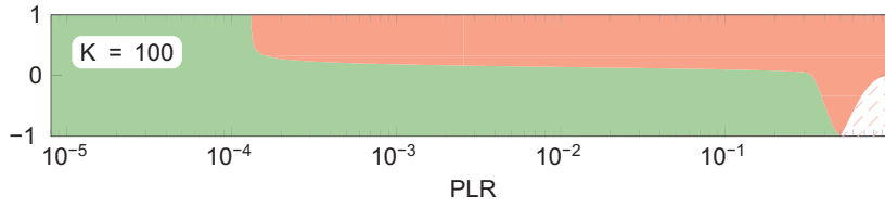
Figure 6.14. Negatively correlating packet losses (y-axis) has a significant impact on control performance. Green area = stable and red area = unstable.
