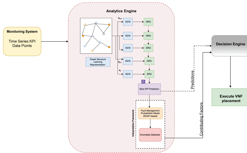
Figure 5.40. Proposed graph-based interpretable anomaly detection (G5IAD) framework.
