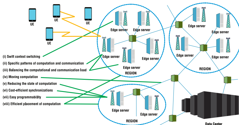
Figure 5.16. Intelligent computation distribution with low-level architectural techniques.
