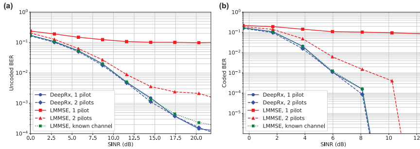
Figure 5.23. DeepRx SIMO reaches linear minimum mean square error (LMMSE) with known channel performance, even for highly mobile UEs of 0–130 km/h as in these figures.
