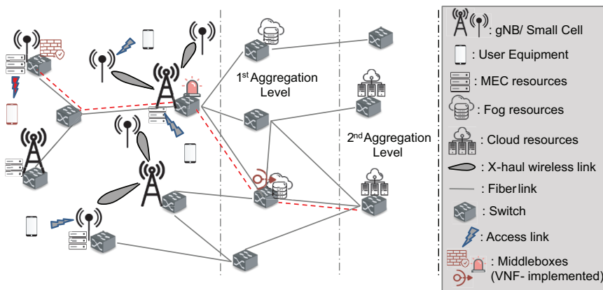
Figure 6.4. Setup overview (in accordance with Figure 6.1) [37].
