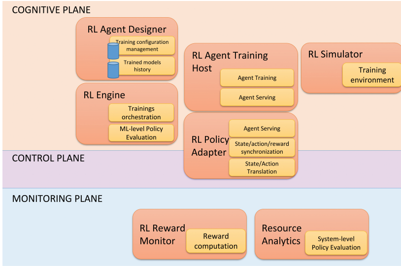
Figure 5.18. Overview of the MA-DRL scheme components.
