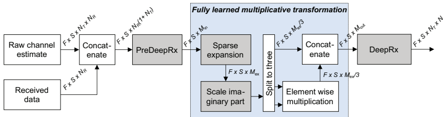
Figure 5.24. DeepRx can be extended to MIMO by adding the capability of input-input multiplication to the neural network, which allows more efficient learned equalization.
