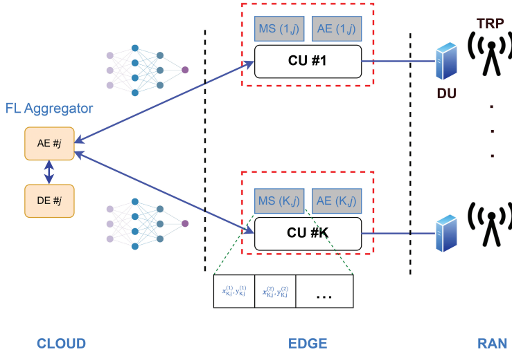
Figure 5.36. Cross-domain statistical FL-based with decentralized MS/AE.
