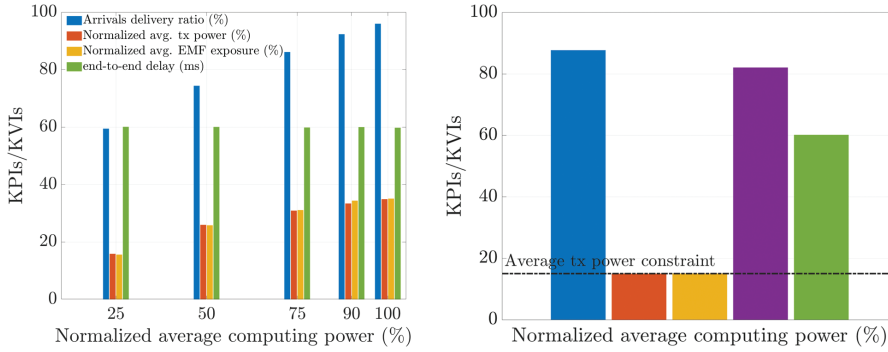
Figure 6.13. Network KPIs/KVIs versus normalized computing power.
