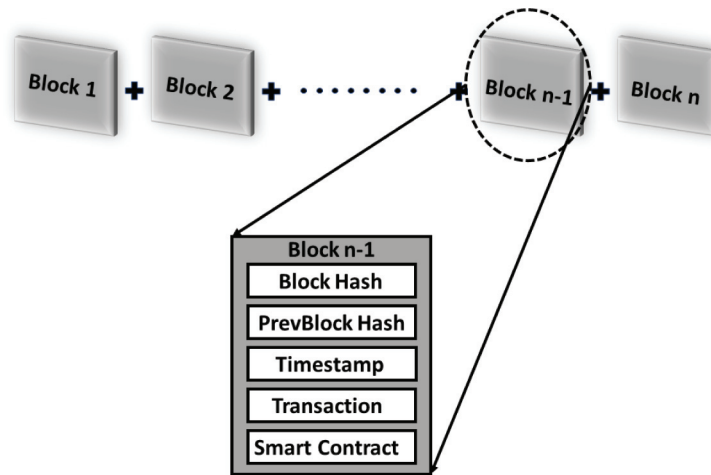
Figure 8.2. An example of a blockchain's ledger.
