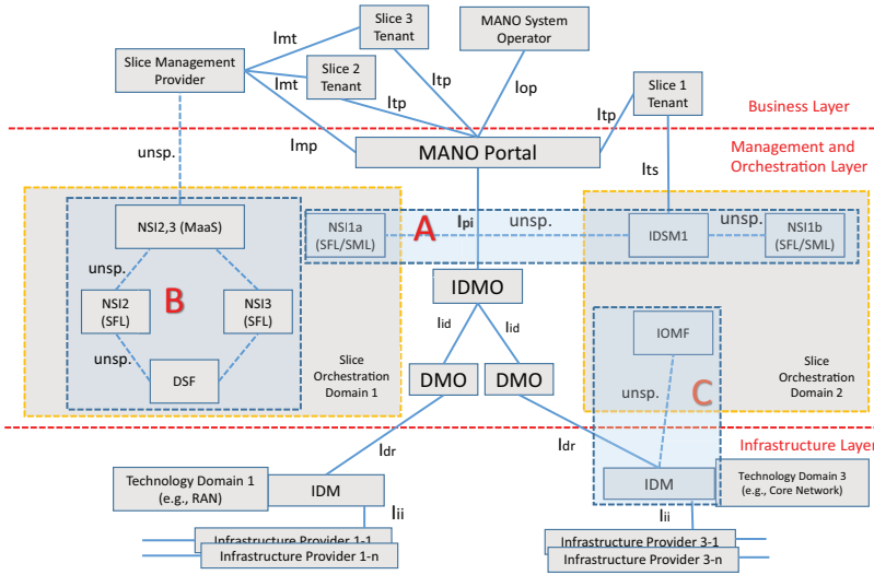
Figure 5.9. Architecture, components and interfaces of the proposed architecture distributed, and scalable MANO framework for 6G evolution.
