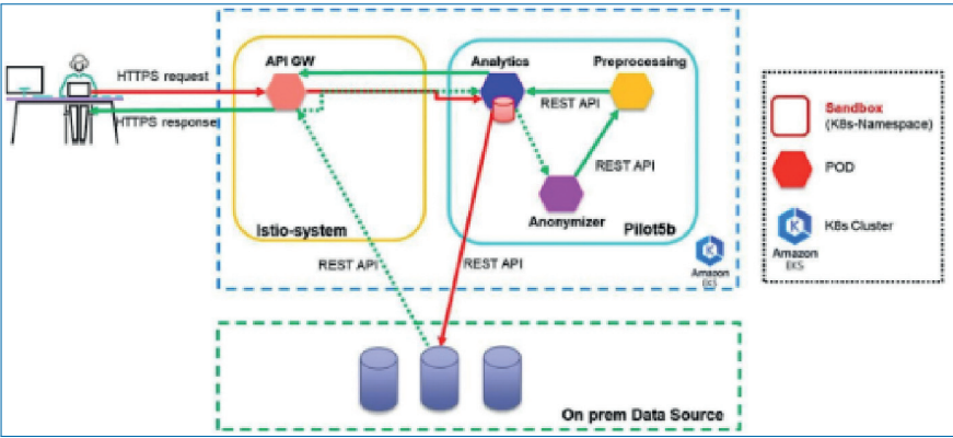
Figure 6.7. Pilot 5b blueprint reference architecture.
